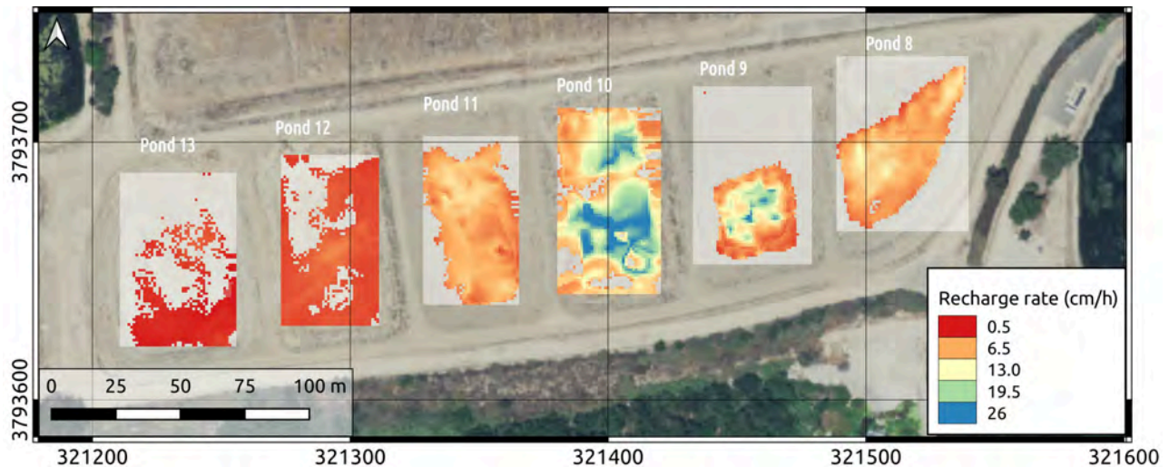
Figure 27. Estimated infiltration rates based on groundwater recharge modeling (Hydrus 1D) for 1 m × 1 m grid cells within each pond, using the K_{sat} distribution estimated from the EMI data.
