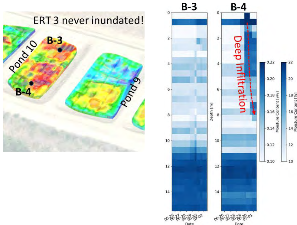
Figure 25. Pond 10 Neutron Probe soil moisture responses for B-3 and B-4. Both B-3 and B-4 are located in sandy soils but B-3 was in the area of the topographic high and was never inundated. Therefore, no changes are observed in the soil moisture along borehole B-3. B-4 shows deep infiltration (red dashed line). Soil moisture increases from ~10% to ~22% from 0-9m bgs. Below 9m soil moisture is somewhat constant.
